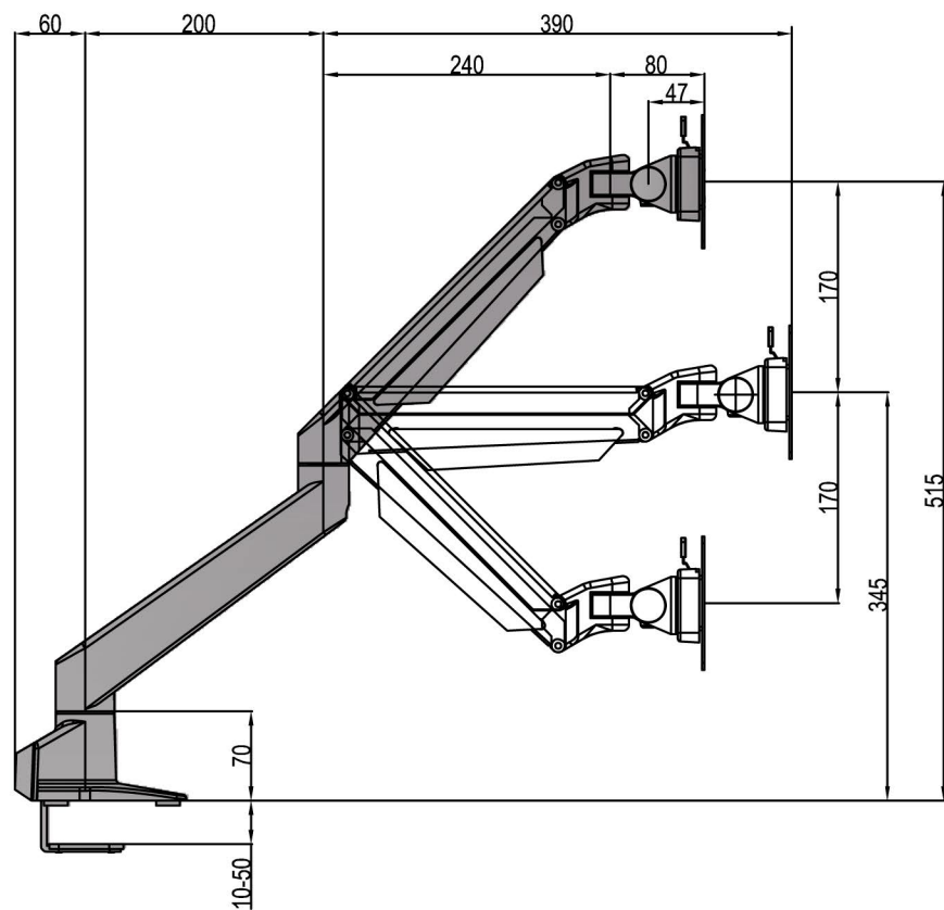
Product Dimensions
